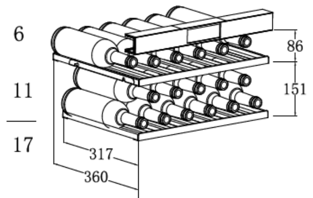
BOTTOM SHELF
