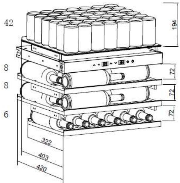
BOTTOM SHELF
