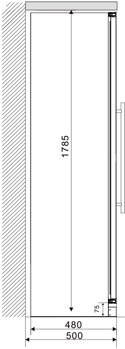
Side View
